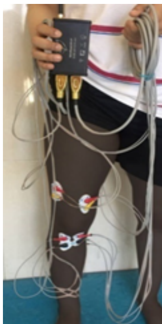
Figure 5. Muscle electromyography
